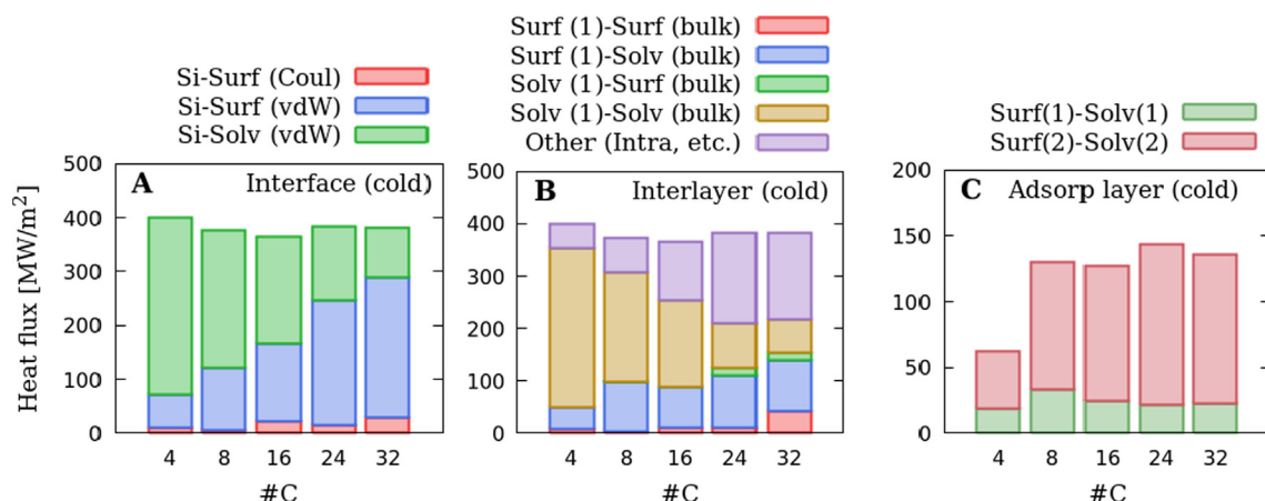
Fig. 7. The interaction contribution to heat flux (A) across the solid–liquid interface, (B) across the liquid–liquid interlayer (Interlayer 1), and (C) between alcohol surfactant and tetracosane solvent in the 1st and 2nd adsorption layers on the cold side for the cases of S-Diol with #C from 4 to 32.
